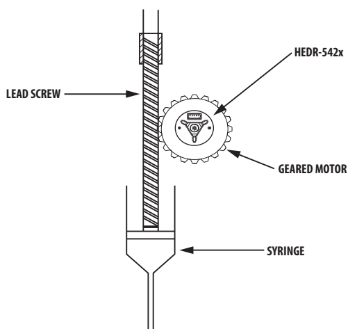
Figure 3. Encoder Used in a Volumetric Dispenser Machine. (drawing not to scale)
