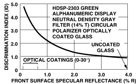
Figure 45. Effect of Reducing Front Surface Reflectance.
