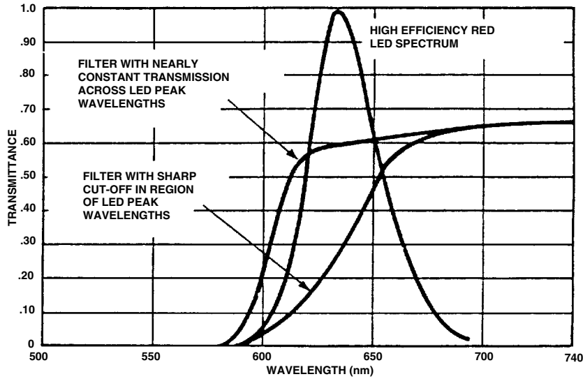
Figure 3. Comparison Between Two Long Pass Red Filters for Use with High-Efficiency Red Displays.
