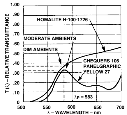
Figure 8. Typical Transmittance Curves for Filters to be used with Yellow Displays.
