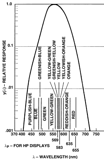
Figure 1. CIE Standard Observer Eye Response Curve (Photopic Curve), including CIE Vivid Color Ranges.
