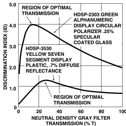
Figure 46. Optimal Neutral Density Gray Filter Transmission.
