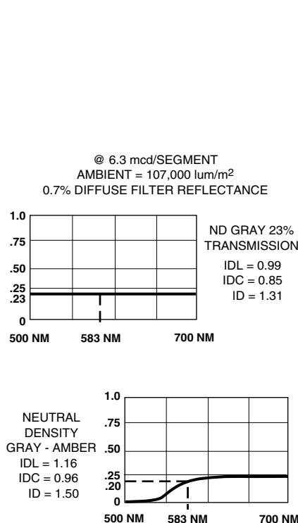
Figure 30. HDSP-4030 Yellow 0.30 inch Display.
