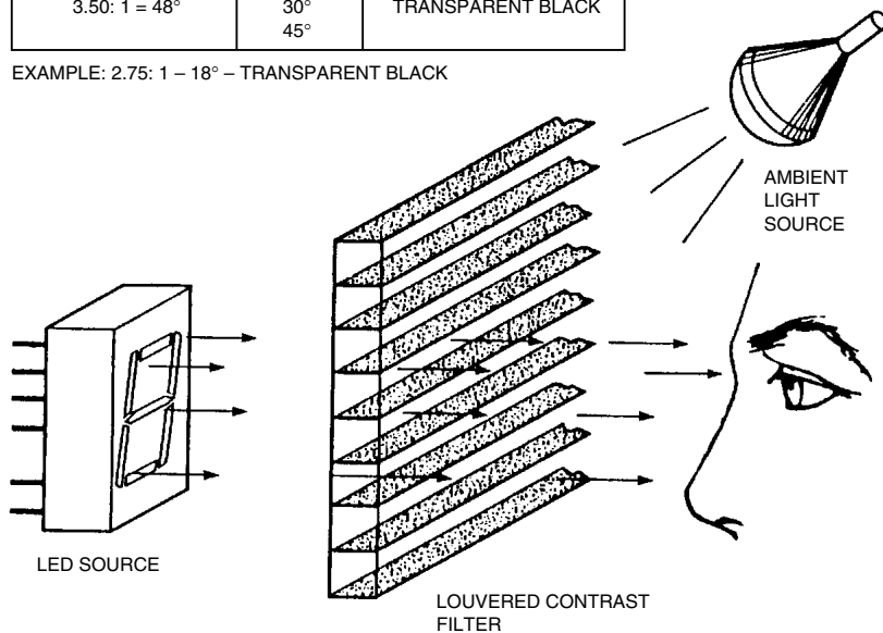
Figure 32. The Operation of a Louvered Filter.
