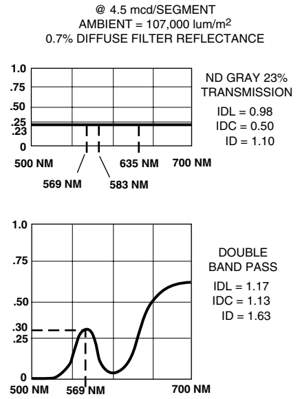
Figure 31. HDSP Green 0.30 inch Display.
