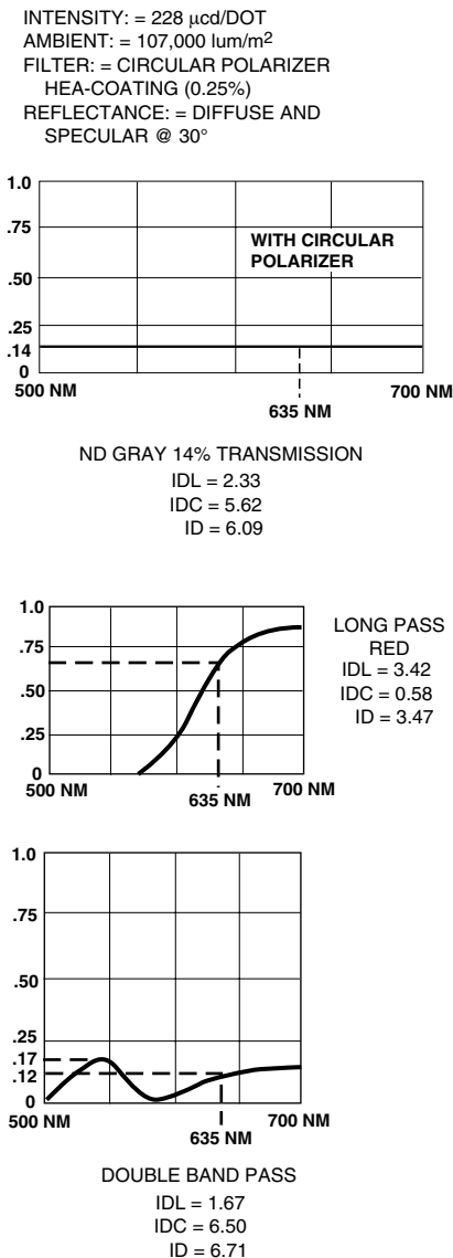
Figure 44. HDSP-2302 High Efficiency Red 0.20 inch Display.
