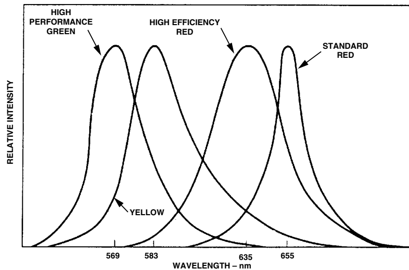
Figure 2. Relative Intensity vs. Wavelength.
