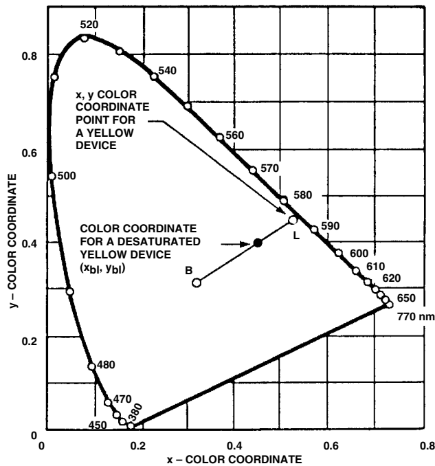
Figure 20. Additive Color Mixture.
