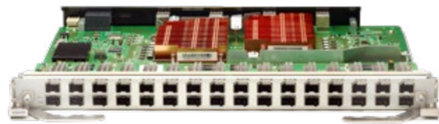
64-port Gen 7 Brocade FC64-64 port blade with 64G line-rate performance
