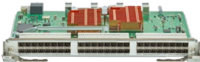
48-port Gen 7 Brocade FC64-48 port blade with 64G line-rate performance
