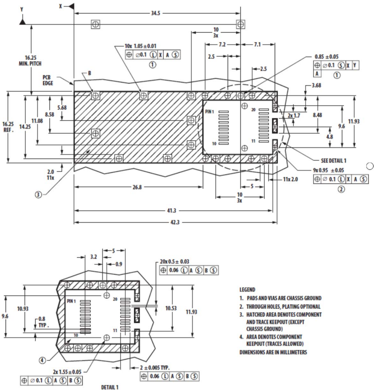
Figure 10. SFP host board mechanical layout
