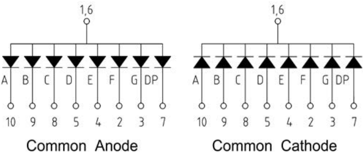
Figure 2: Circuit Diagram
