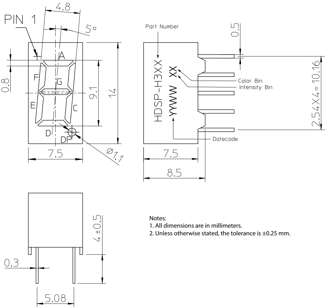
Figure 1: Package Dimension
