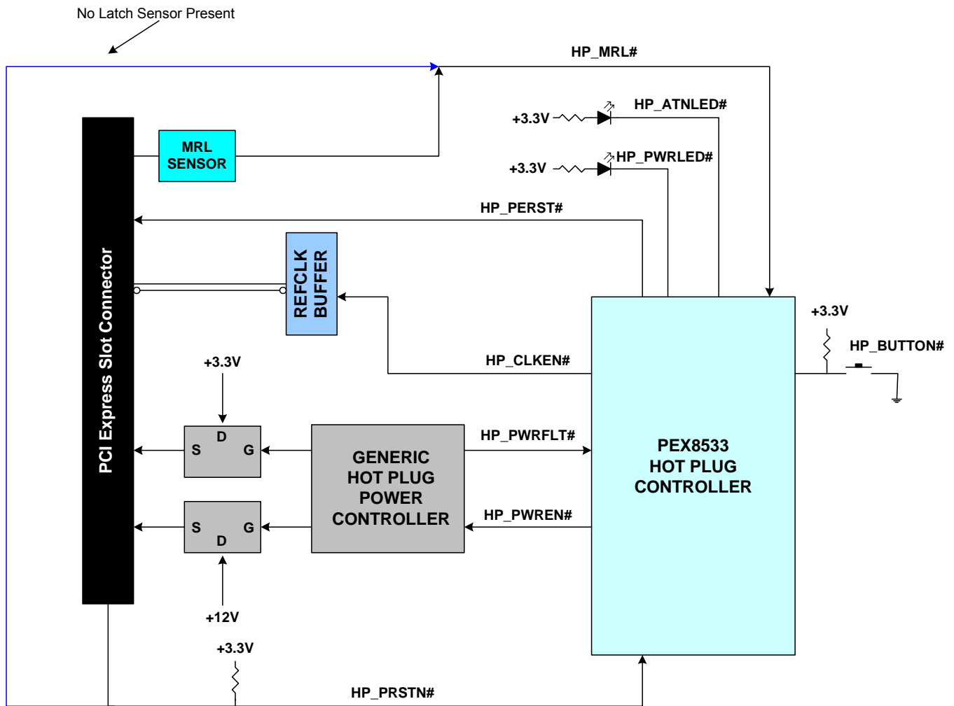
Figure 6. PEX 8533 Hot Plug Controller Interface
