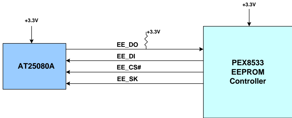
Figure 4. PEX 8533 1-Kbyte SPI EEPROM Interface
