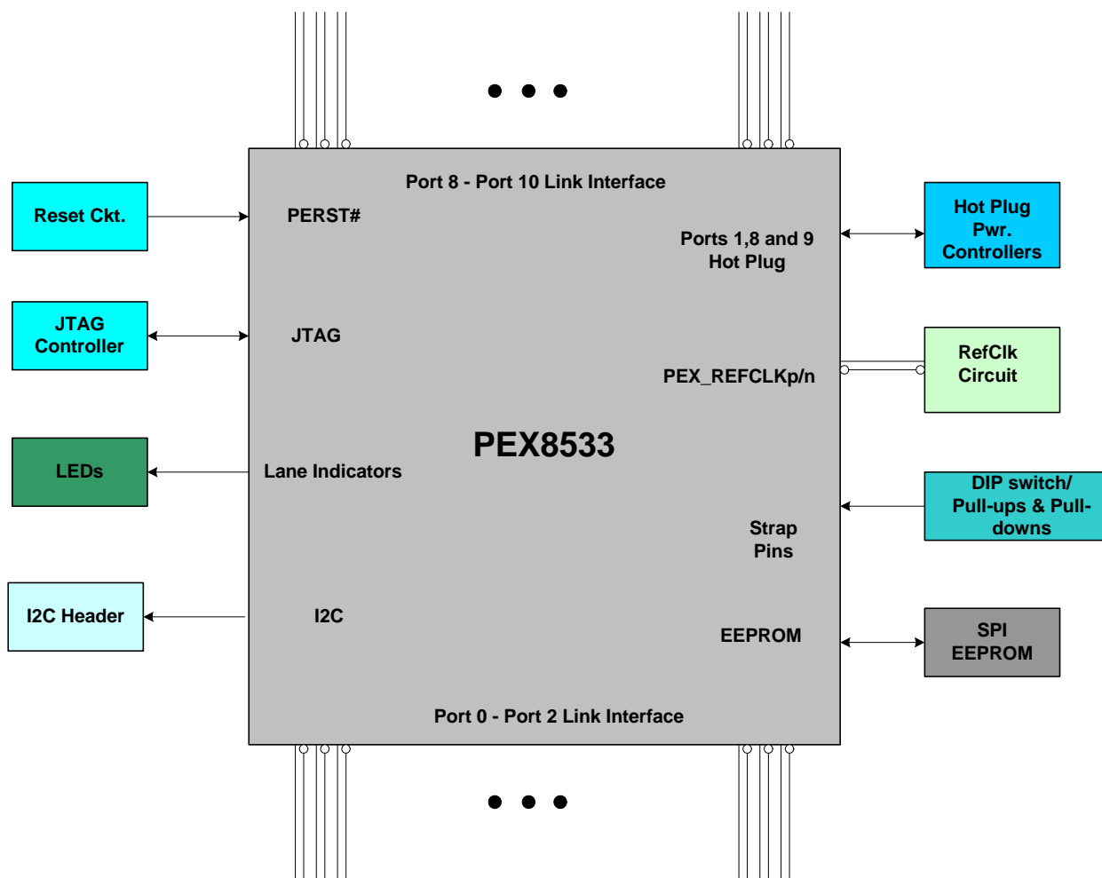
Figure 1. PEX 8533 Interfaces
