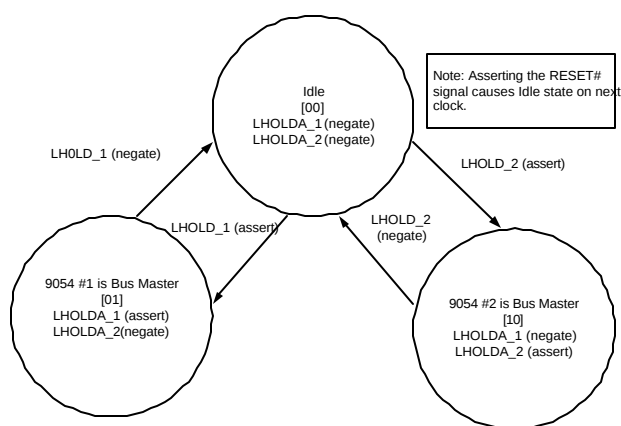
Figure 2. State Diagram of Local Bus Arbiter
