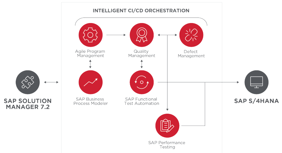
Figure 1: SAP Platform
