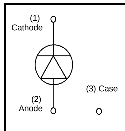
ELED Pinout
