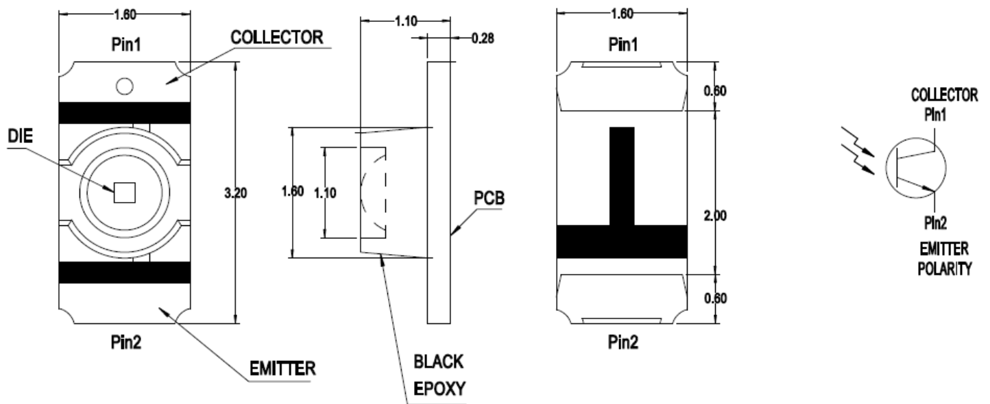
Figure 1: Package Drawing
