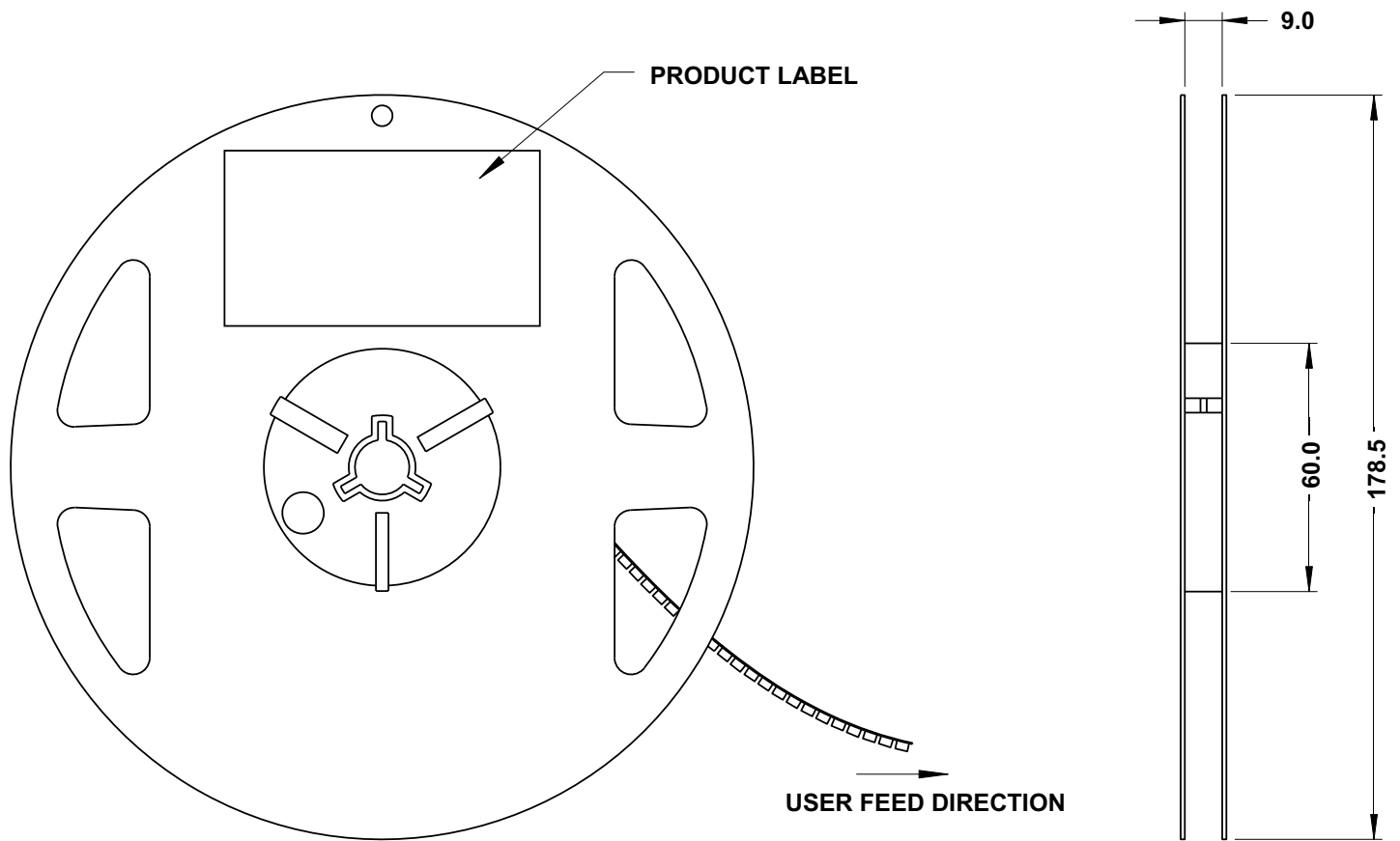
Figure 10: Reel Dimensions
