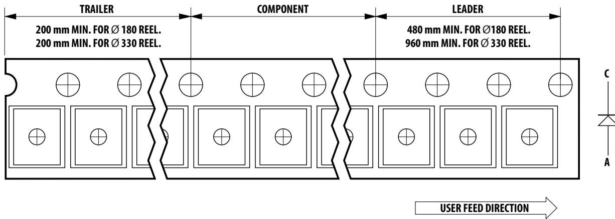
Figure 12: Tape Dimensions
