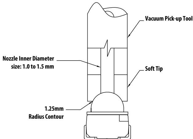
Figure 9: Soft Tip Vacuum Pick-Up Tool for Extracting SMD LED Components from Carrier Tape
