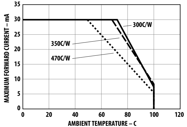
Figure 6: Maximum Forward Current vs. Ambient Temperature. Derated Based on TJmax = 110 °C (InGaN)
