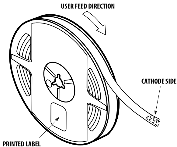
Figure 13: Reeling Orientation
