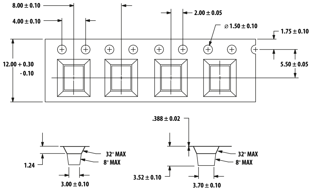
Figure 12: Tape Dimensions
