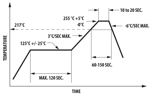
Figure 10: Recommended Pb-Free Reflow Soldering Profile
