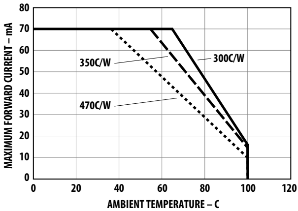
Figure 5: Maximum Forward Current vs. Ambient Temperature. Derated Based on TJmax = 110 °C (AllInGaP)
