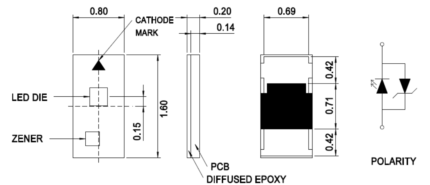
Figure 1: Package Dimensions
