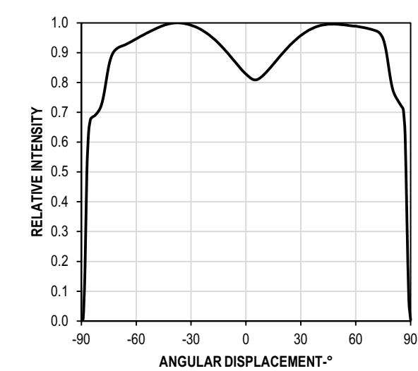
Figure 5: Intensity vs. Angle
