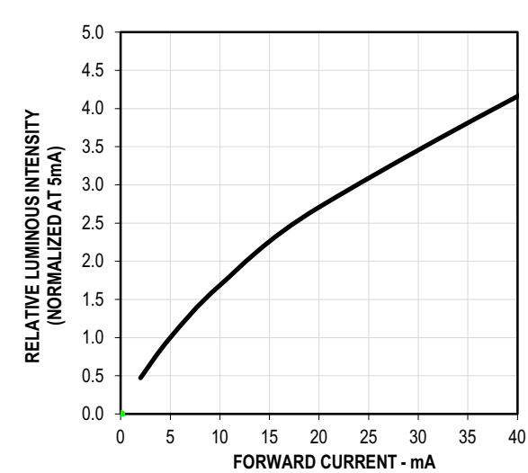
Figure 4: Intensity vs. Forward Current
