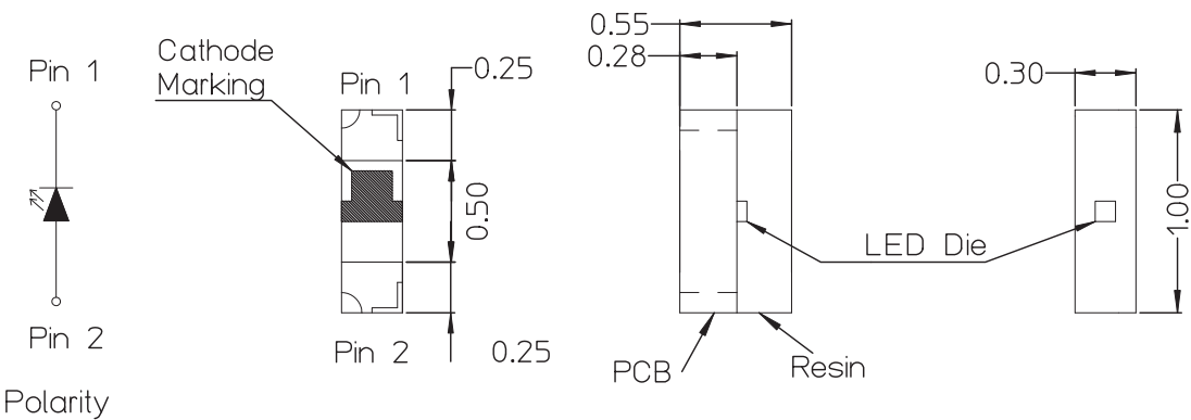
Figure 1: Package Dimensions
