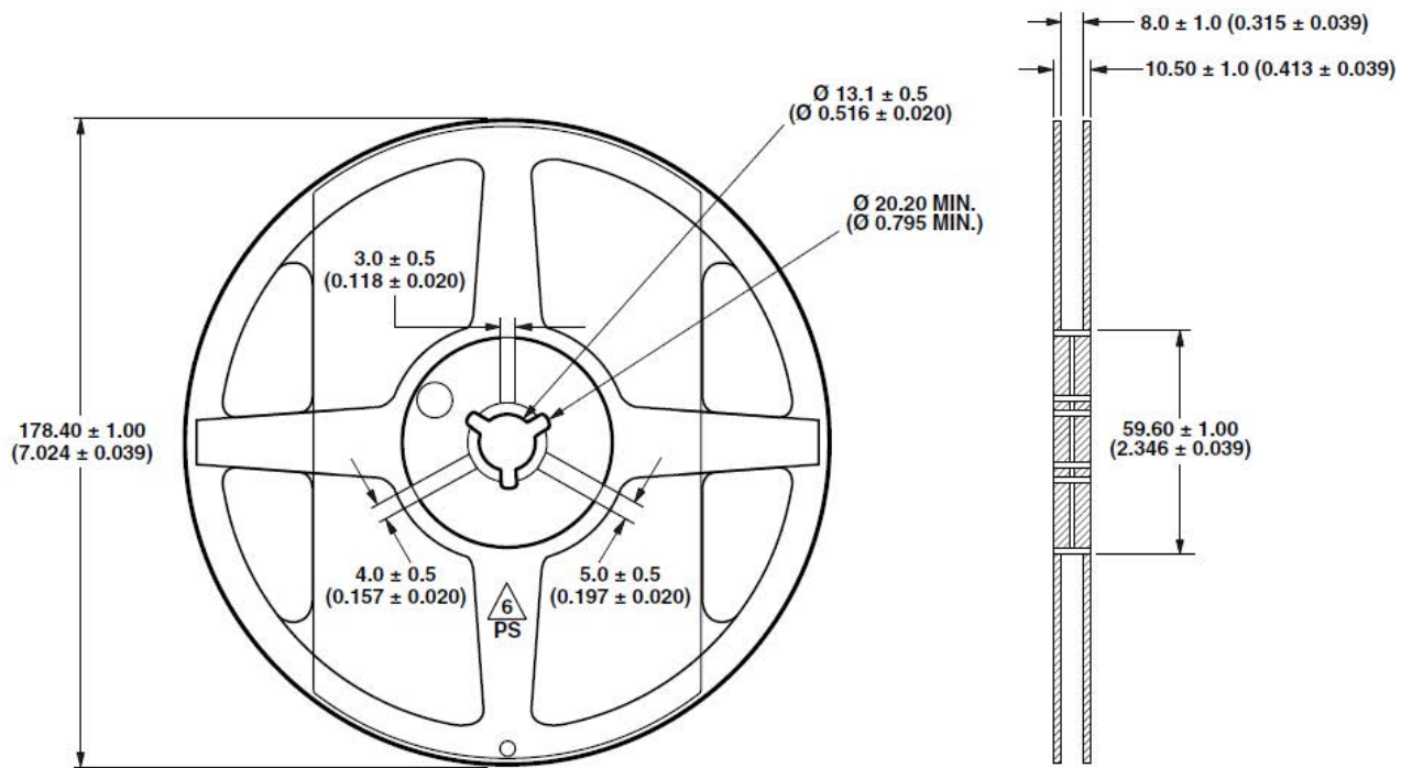
Figure 12: Reel Dimensions
