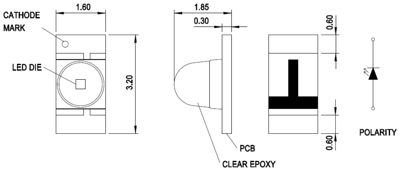
Figure 1: Package Dimensions
