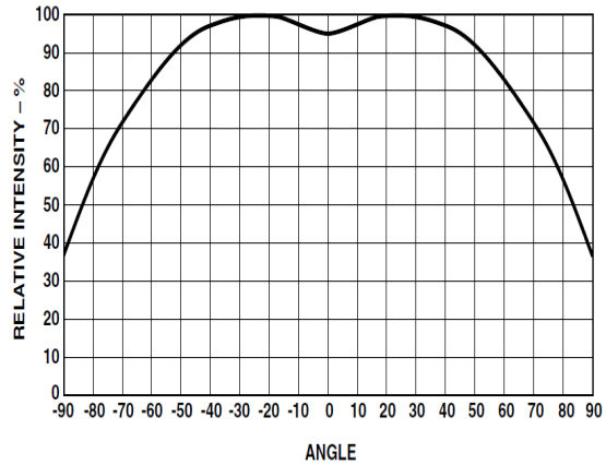
Figure 5: Radiation Pattern
