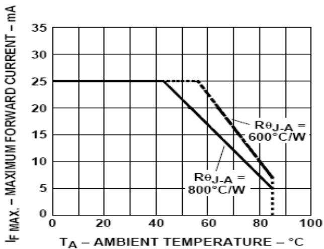
Figure 6: Derating Curve
