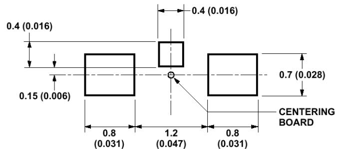
Figure 7: Recommended Soldering Land Pattern
