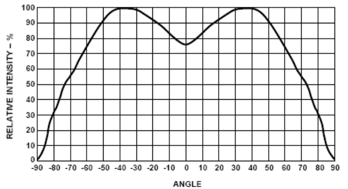
Figure 5: Radiation Pattern
