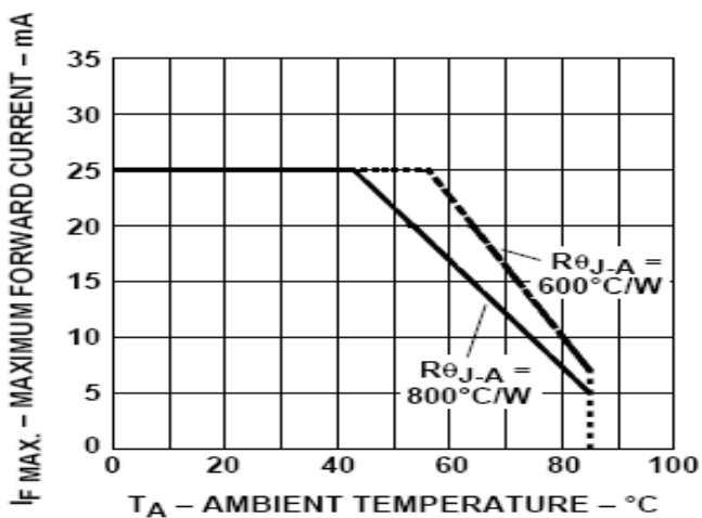
Figure 6: Derating Curve
