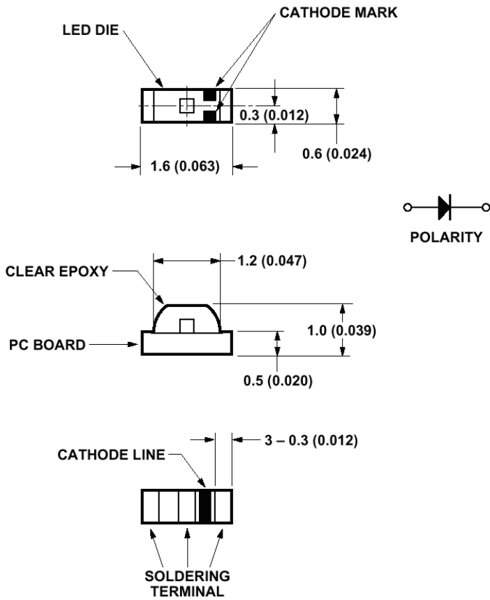
Figure 1: Package Dimensions
