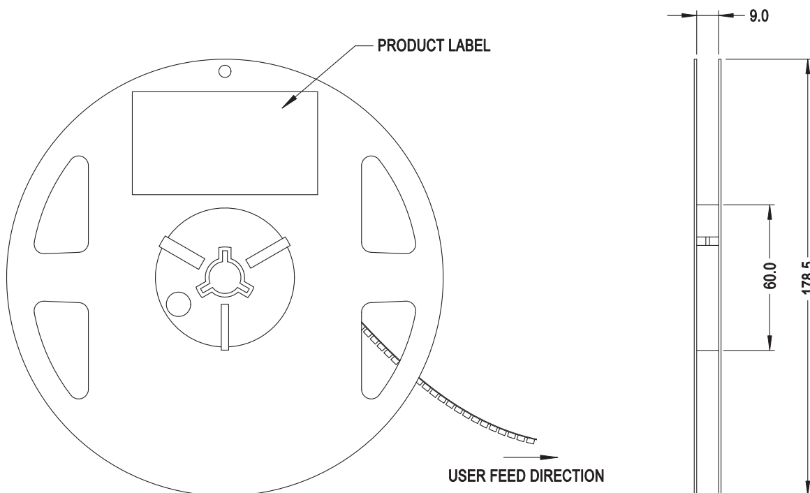
Figure 8: Reel Dimensions
