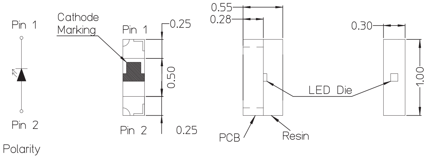
Figure 1: Package Dimensions
