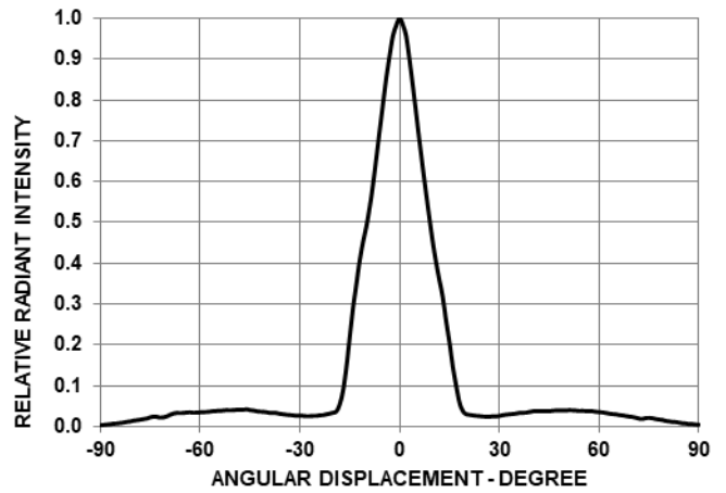
Figure 4: Radiation Pattern
