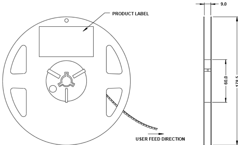
Figure 8: Reel Dimensions
