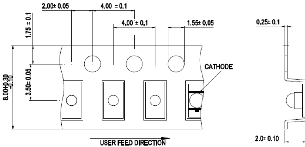
Figure 7: Carrier Tape Dimensions
