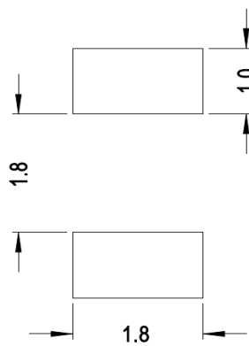
Figure 6: Recommended Soldering Land Pattern
