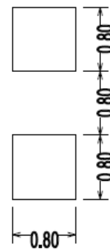
Figure 7: Recommended Soldering Land Pattern
