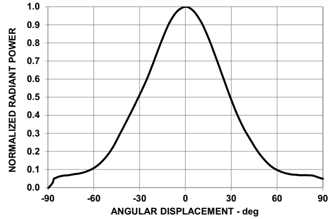
Figure 5: Radiation Pattern
