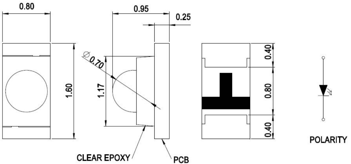
Figure 1: Package Dimensions
