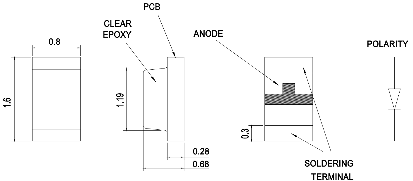
Figure 1: Package Dimensions
