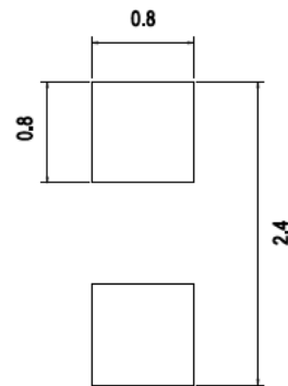
Figure 7: Recommended Soldering Land Pattern
