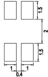
Figure 5: Recommended Soldering Land Pattern
