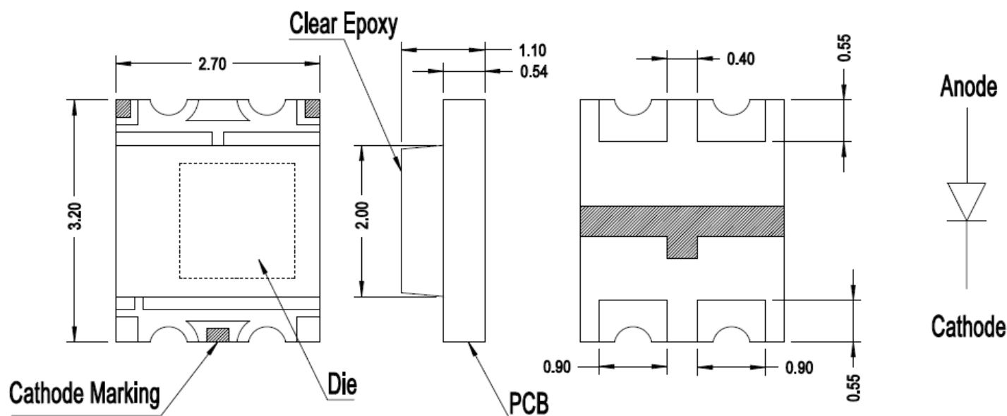
Figure 1: Package Drawing
