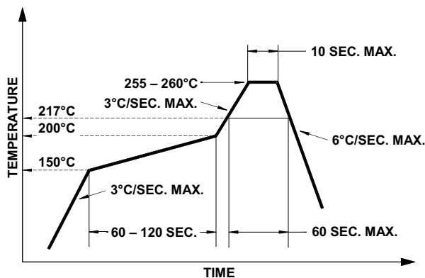
Figure 8: Recommended Lead-Free Reflow Soldering Profile
