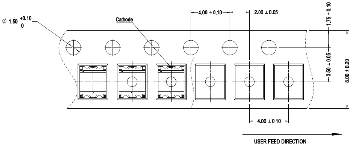
Figure 6: Carrier Tape Dimensions
