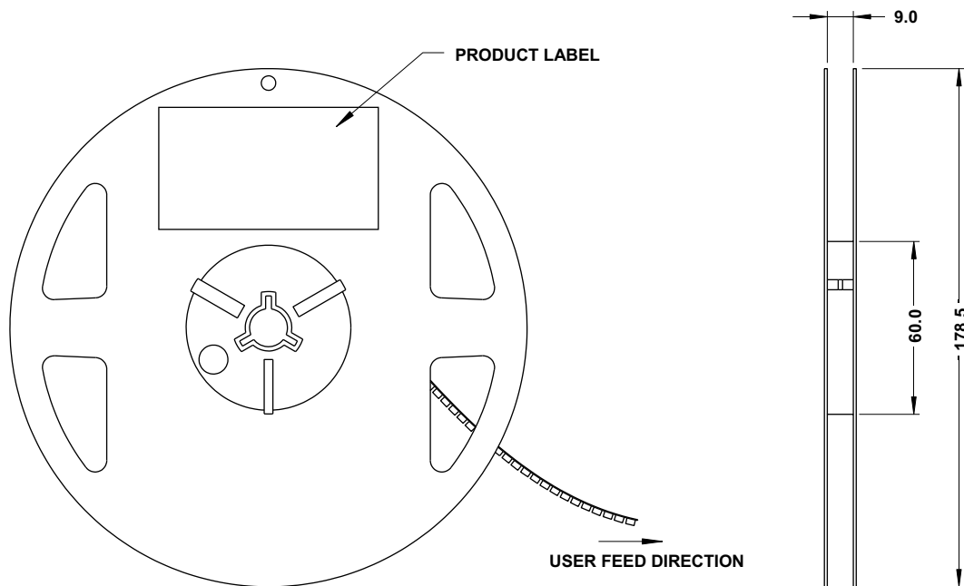
Figure 7: Reel Dimensions
