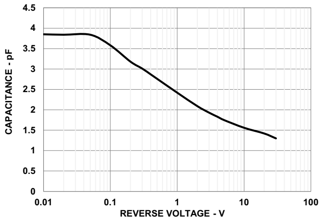
Figure 5: Diode Capacitance vs. Reverse Voltage ( E_e = 0\text{mW/cm}^2 , f = 1\text{ MHz} )
