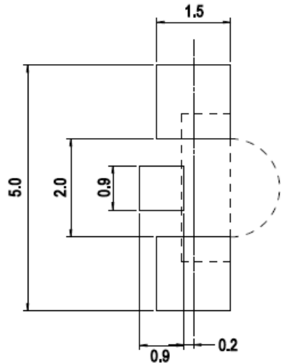
Figure 6: Recommended Soldering Land Pattern
