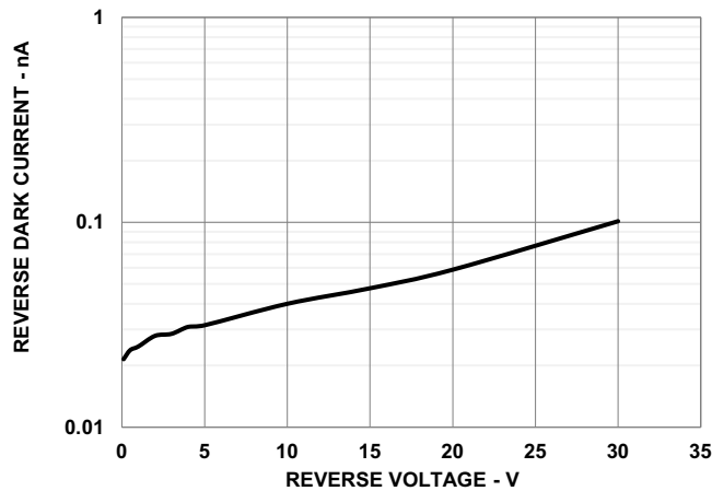
Figure 4: Reverse Dark Current vs. Reverse Voltage ( E_e = 0\text{mW/cm}^2 )
