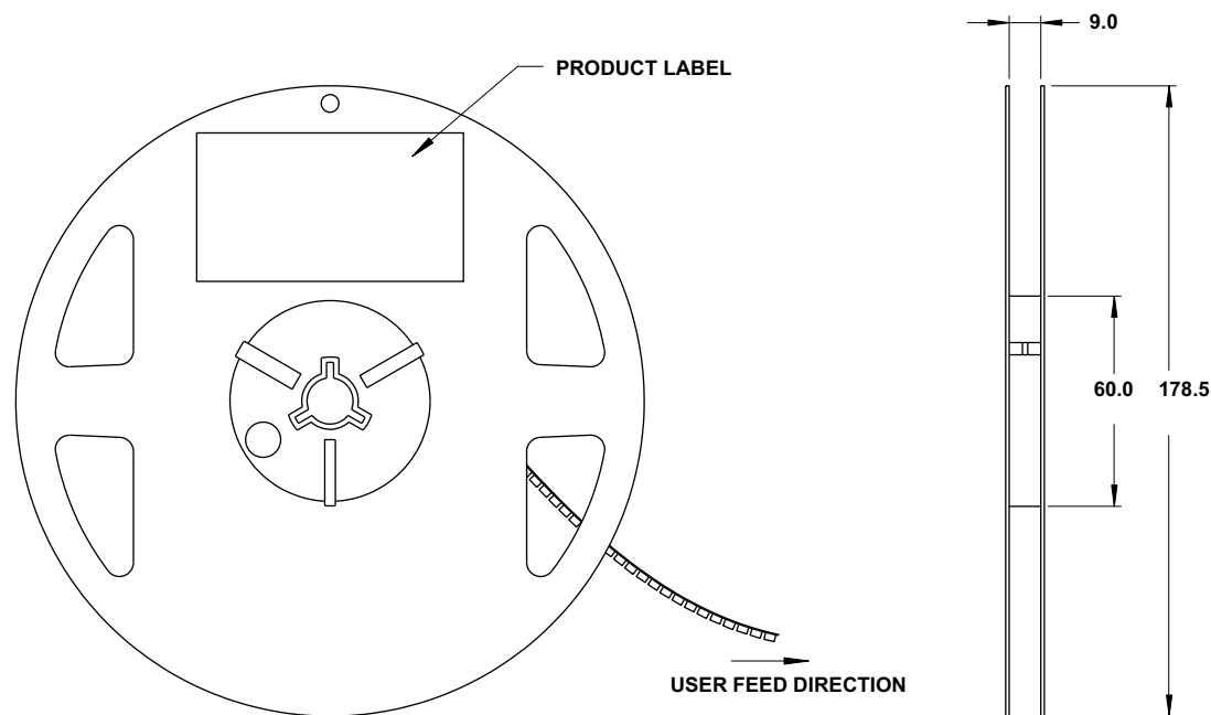
Figure 8: Reel Dimensions
