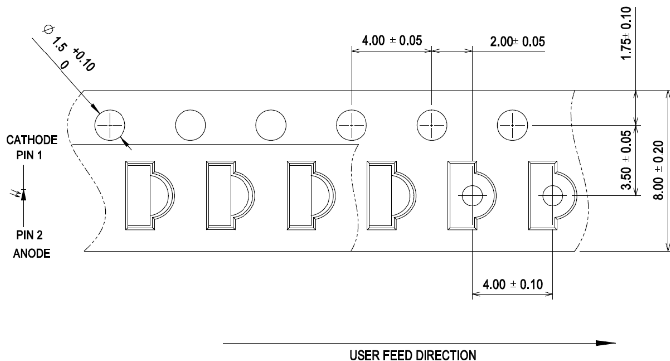
Figure 7: Carrier Tape Dimensions
