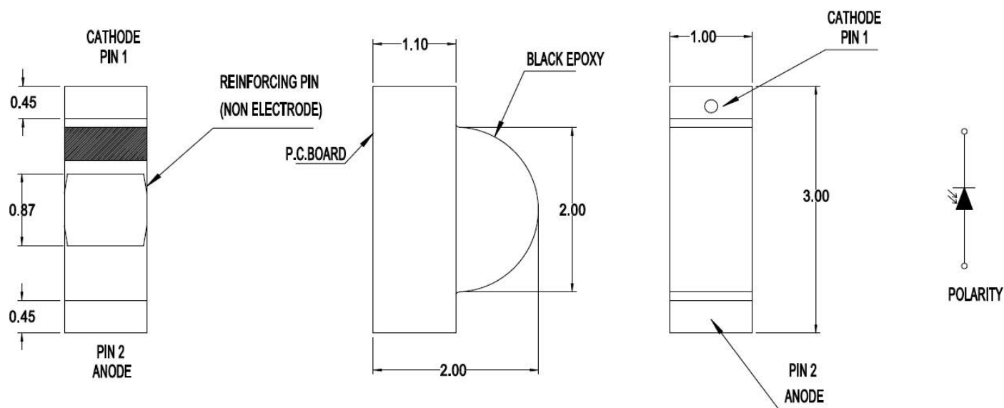
Figure 1: Package Drawing
