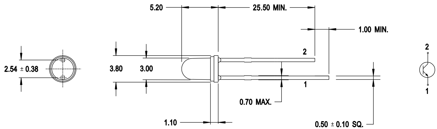
Figure 1: Package Drawing
