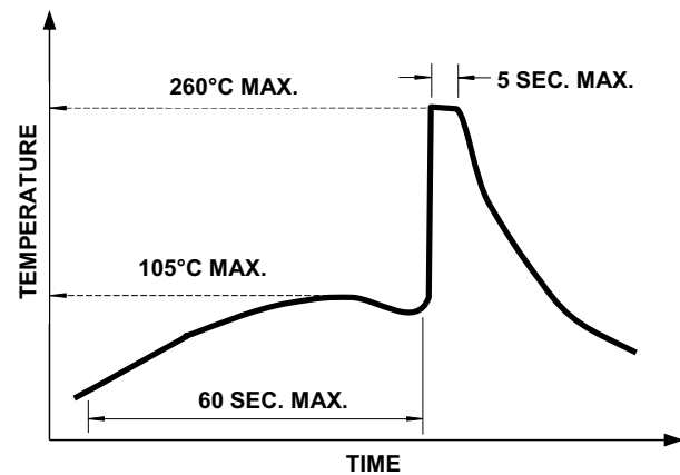
Figure 11: Recommended Wave Soldering Profile
