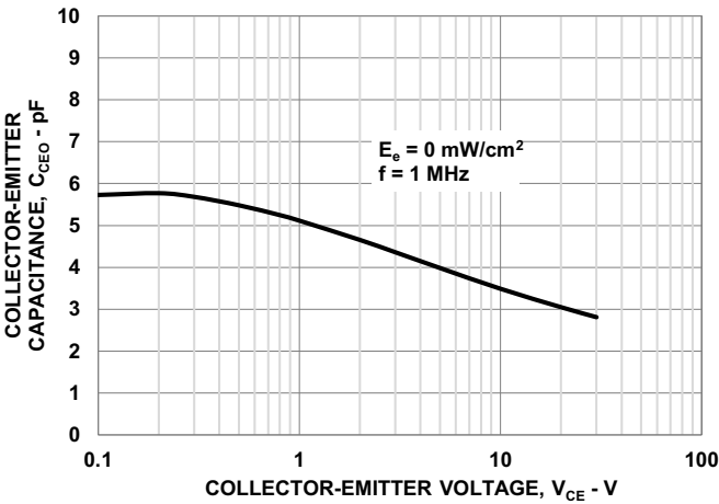
Figure 8: Collector-Emitter Capacitance vs. Collector-Emitter Voltage
