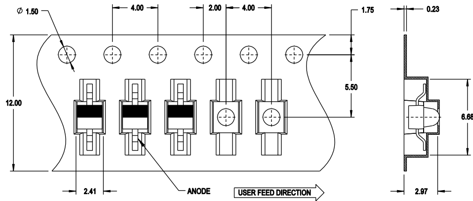
Figure 12: Carrier Tape Dimensions for Z-Bend Lead
