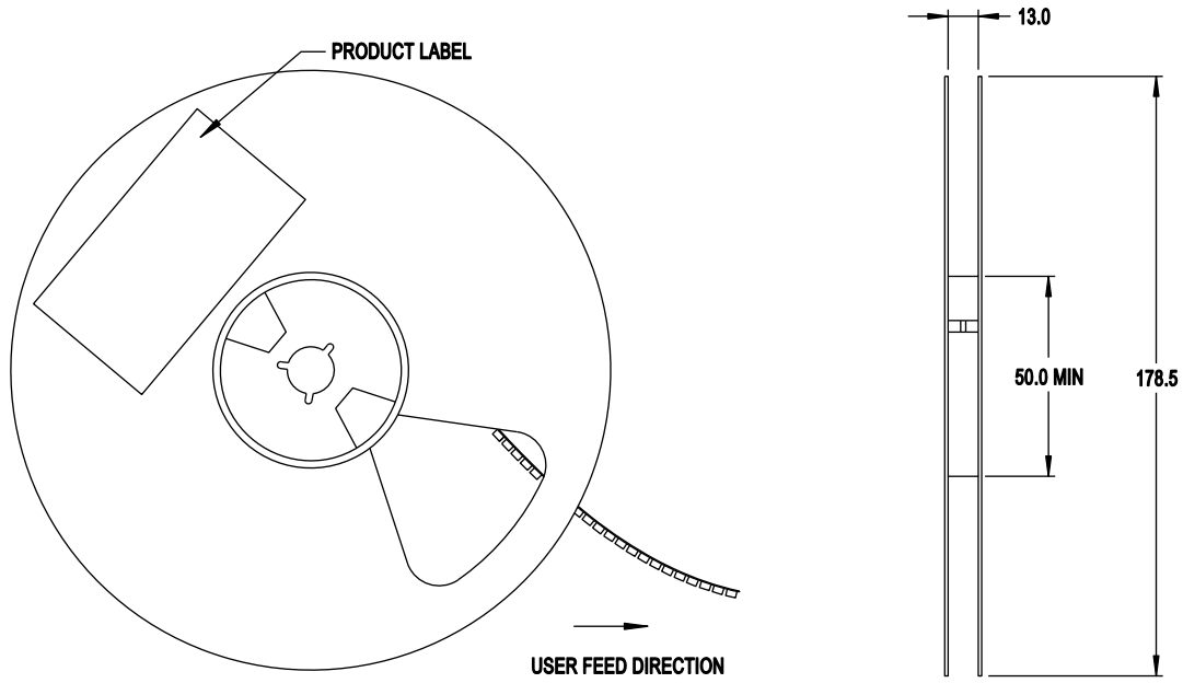
Figure 13: Reel Dimensions (7-inch Tape and Reel)
