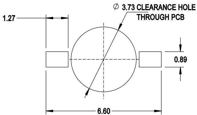
Figure 10: Recommended Soldering Land Pattern for Z-Bend Lead
