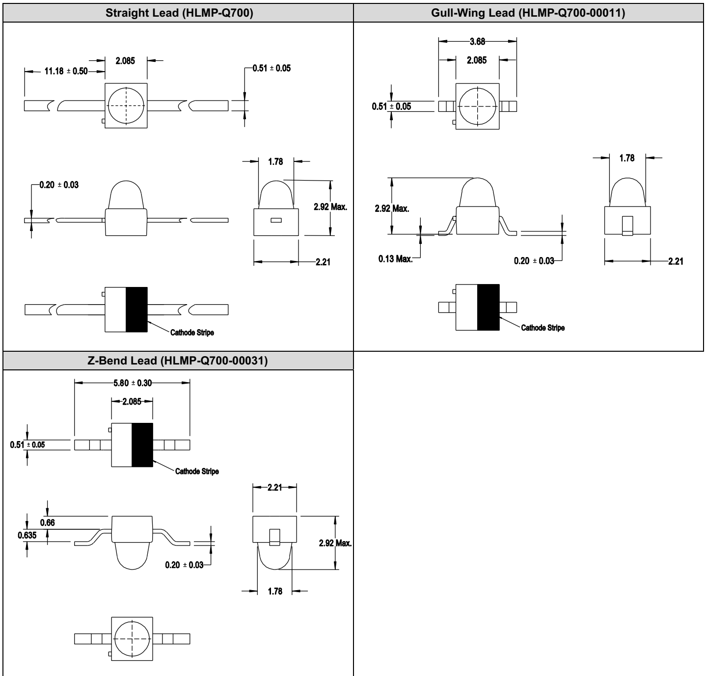
Figure 1: Package Drawing
