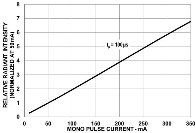
Figure 4: Relative Radiant Intensity vs. Mono Pulse Current
