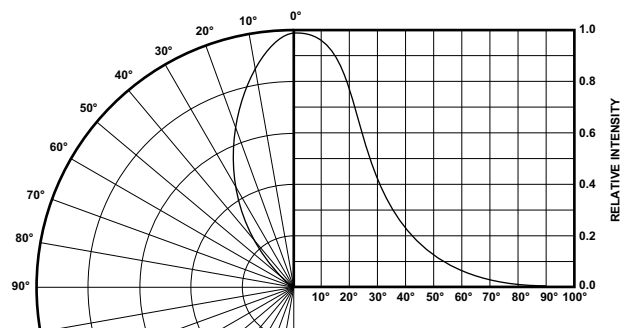
Figure 6: Relative Illuminous Intensity vs. Angular Displacement for T-1 Lamp
