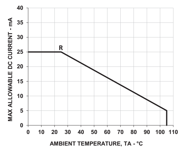
Figure 11: Allowable DC Current vs. Ambient Temperature
