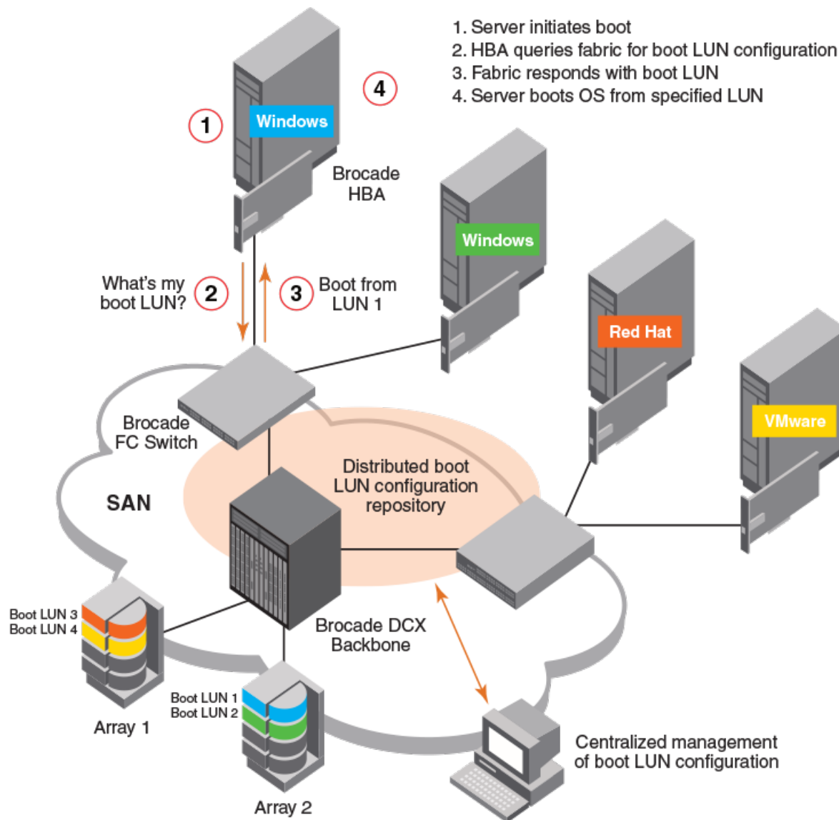
Figure 59: Boot LUN Zoning
