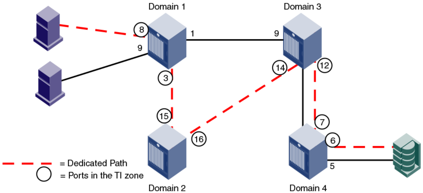
Figure 63: Dedicated Path is Not the Shortest Path
