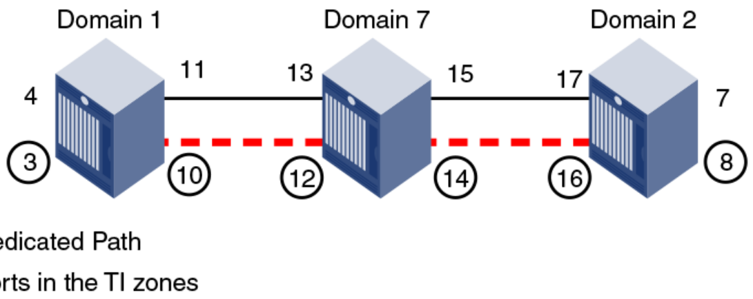
Figure 75: Creating a TI Zone in a Base Fabric
