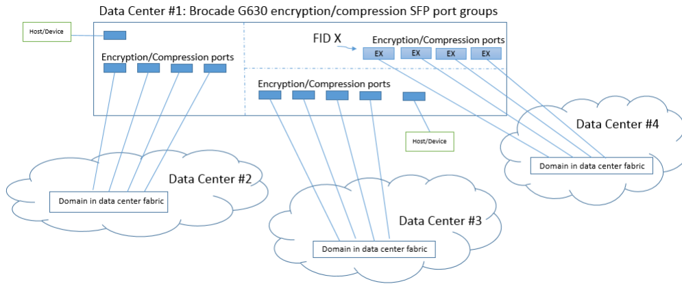
Figure 20: Unsupported Configuration with FCR
