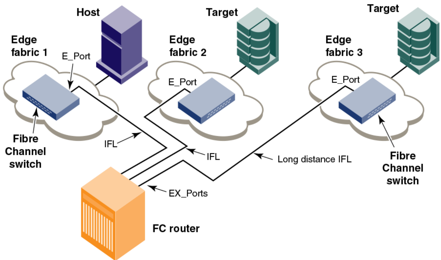
Figure 84: A metaSAN with Inter-Fabric Links
