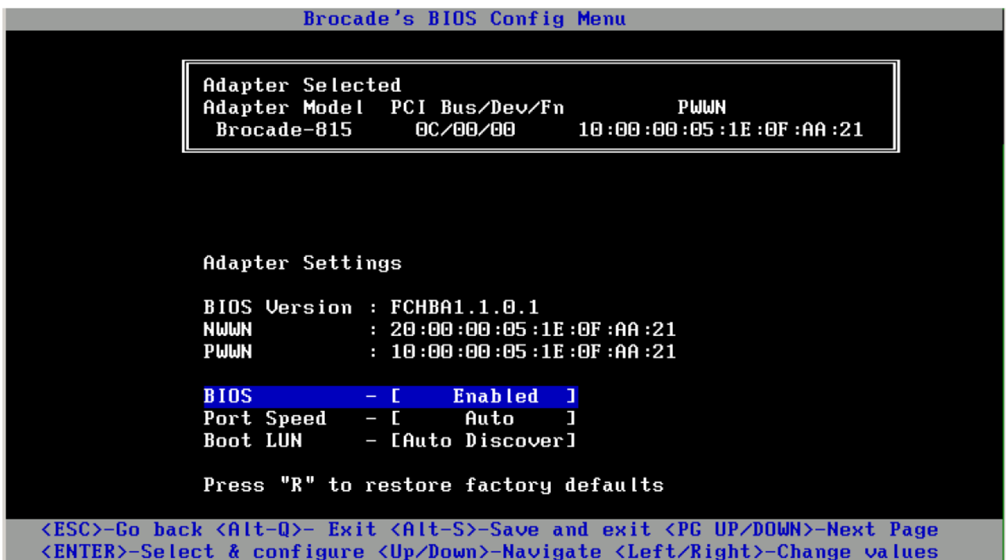
Figure 60: Boot LUN Zoning BIOS Setting
