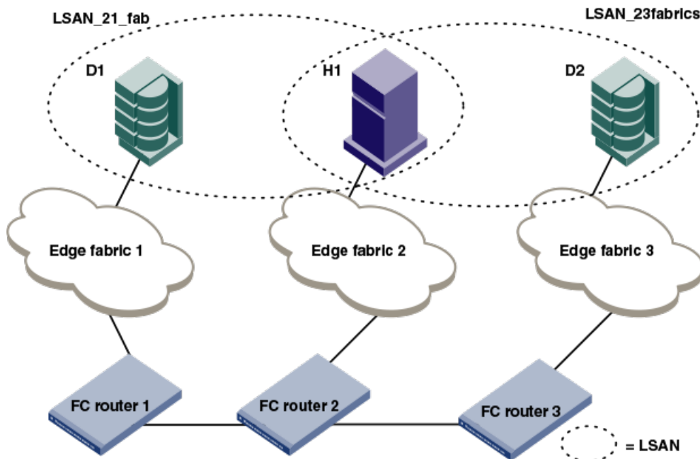
Figure 91: Example of Setting up Enforce LSAN Tag
