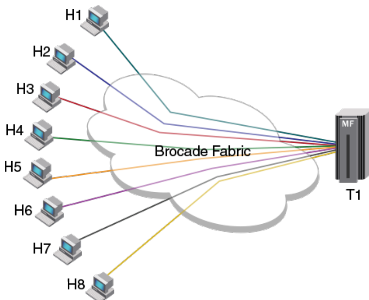
Figure 54: Single-Initiator Zoning Example
