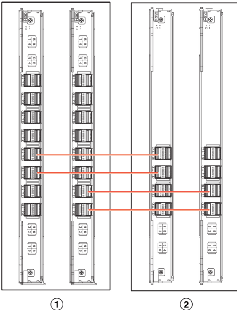
Figure 33: Minimum Configuration for 128Gb/s ICLs
