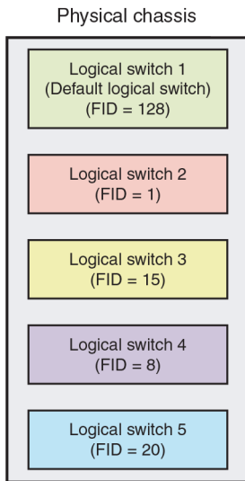
Figure 44: Fabric IDs Assigned to Logical Switches
