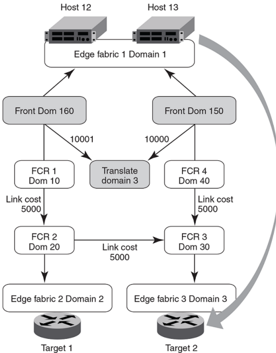
Figure 90: Shortest IFL Solution
