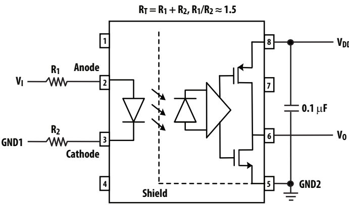
Figure 14: Recommended Drive Circuit for High CMR
