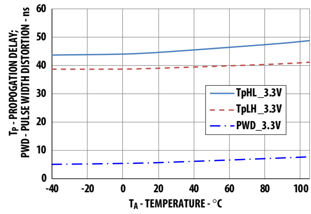
Figure 10: Typical Switching Speed versus Temperature at 3.3V Supply Voltage
