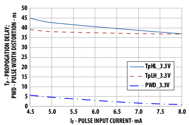
Figure 8: Typical Switching Speed versus Pulse Input Current at 3.3V Supply Voltage
