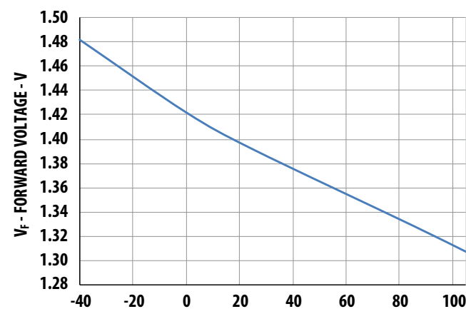
Figure 3: Typical V_F versus Temperature
