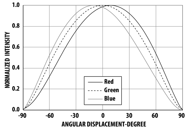
Figure 12: Radiation Pattern along Y-axis of the Package
