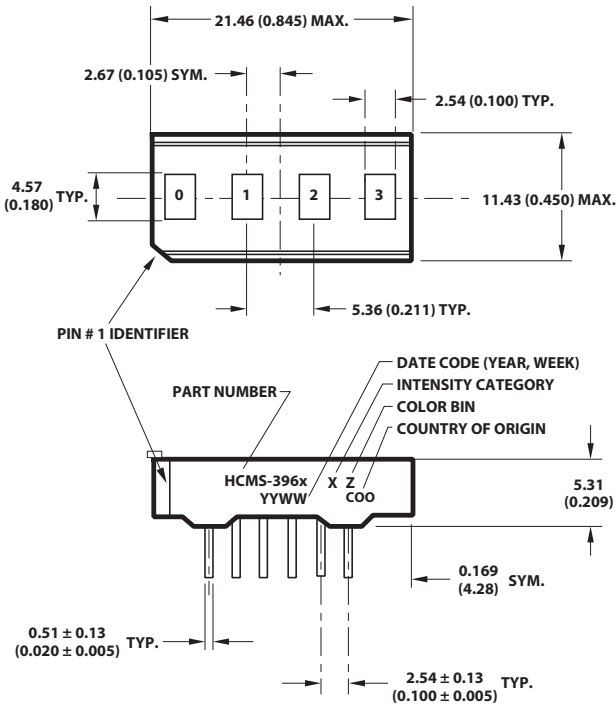
Figure 3: HCMS-396X Package Dimensions
