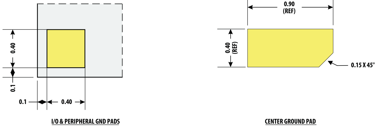
Figure 24. Pad Detail
