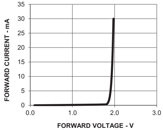
Figure 14: Forward Current vs. Forward Voltage
