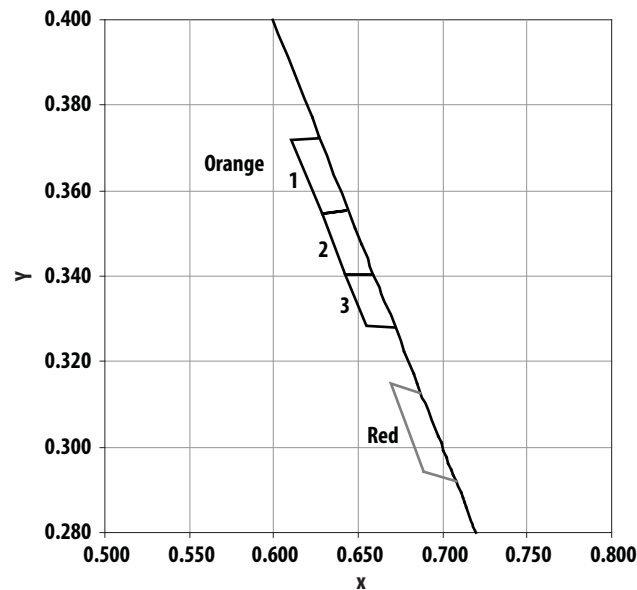
Avago Color Bin on CIE 1931 Chromaticity Diagram
