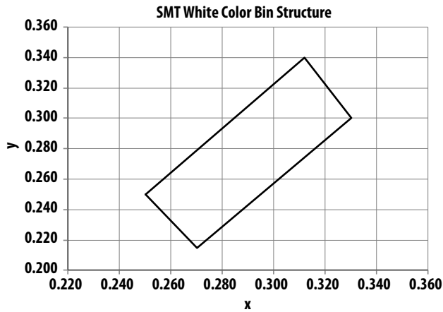
Figure 1: Color Bin Limit (CIE 1931 Chromaticity Diagram) [Tolerance: ± 0.02]
