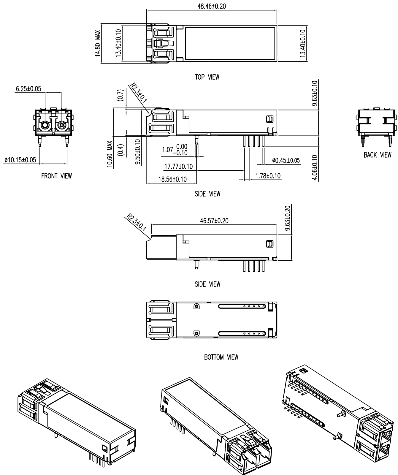
Figure 4. AFCT-5941xTxZ Package Outline Drawing
