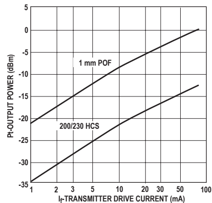
Figure 4. Typical Transmitter Output Power vs. Drive Current.
