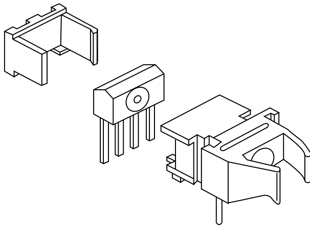
Figure 2. Package Construction.
