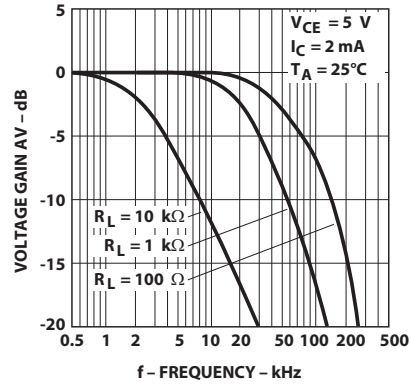
Figure 10: Frequency Response
