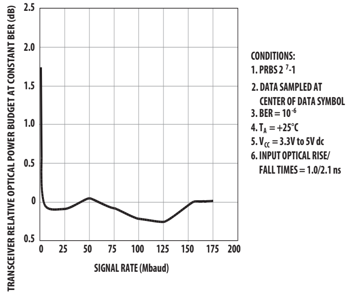
Figure 7: Transceiver Relative Optical Power Budget at Constant BER vs. Signaling Rate
