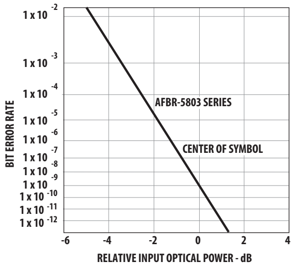
Figure 8: Bit Error Rate vs. Relative Receiver Input Power
