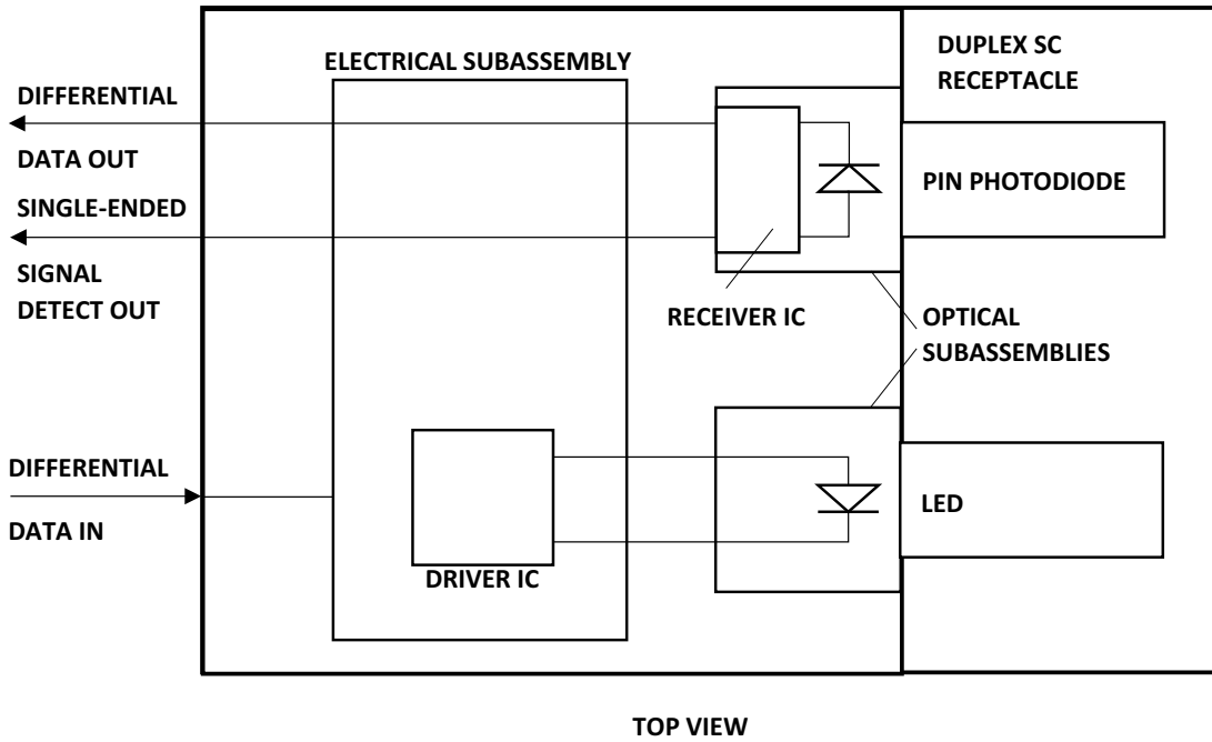
Figure 1: SC Connector Block Diagram
