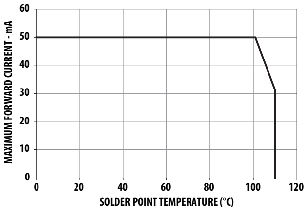
Figure 5: Maximum Forward Current vs. Solder Point Temperature, Derated Based on T_{JMAX}=125^{\circ}C , R_{\theta J-A}=110^{\circ}C/W
