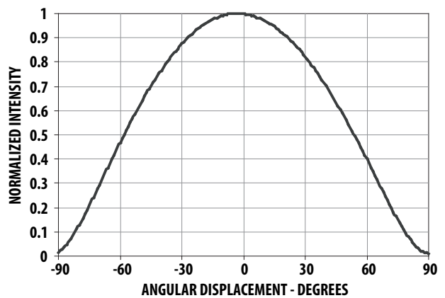
Figure 6: Radiation Pattern
