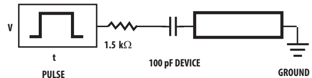
Figure 1: Human-Body ESD Circuit Model
