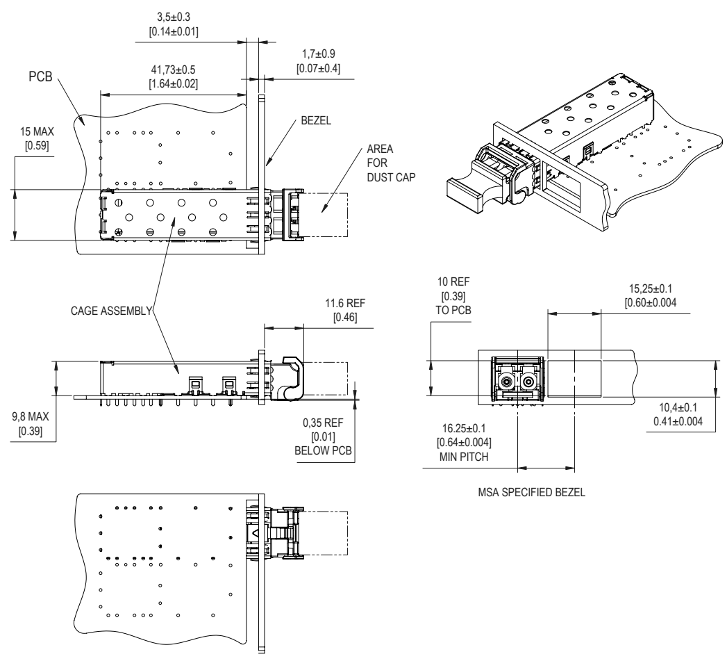
Figure 6. Module Drawing
