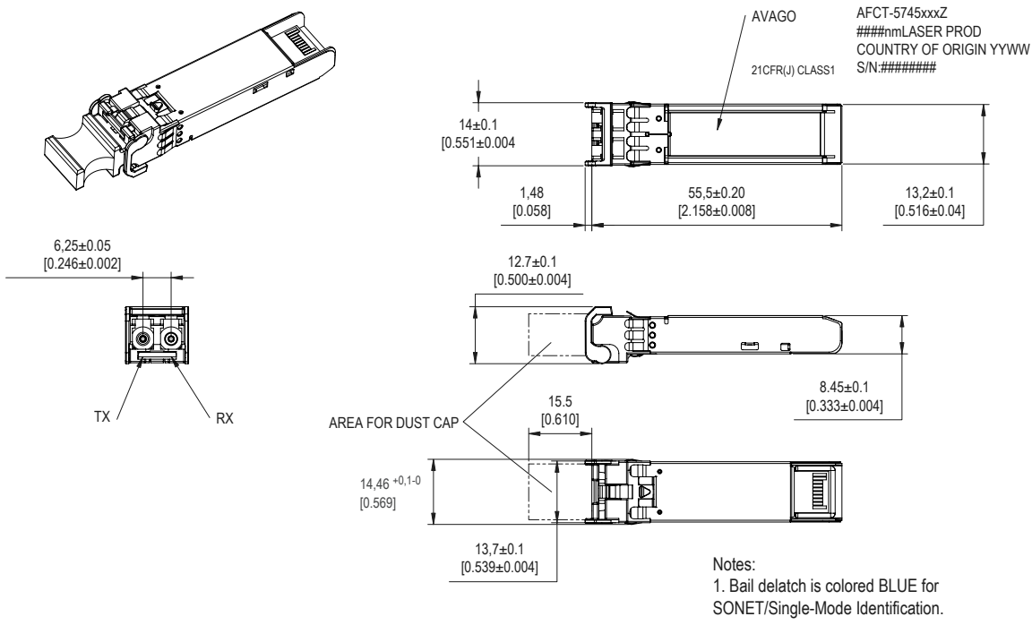
Figure 6. Module Drawing
