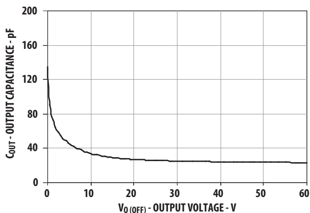
Figure 6: Output Capacitance vs. Output Voltage
