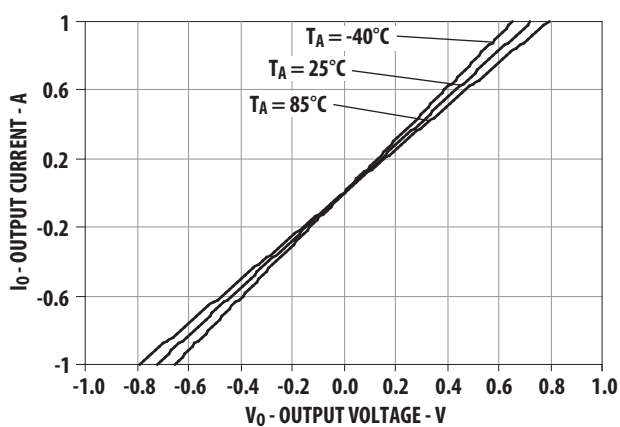
Figure 10: Typical Output Current vs. Output Voltage
