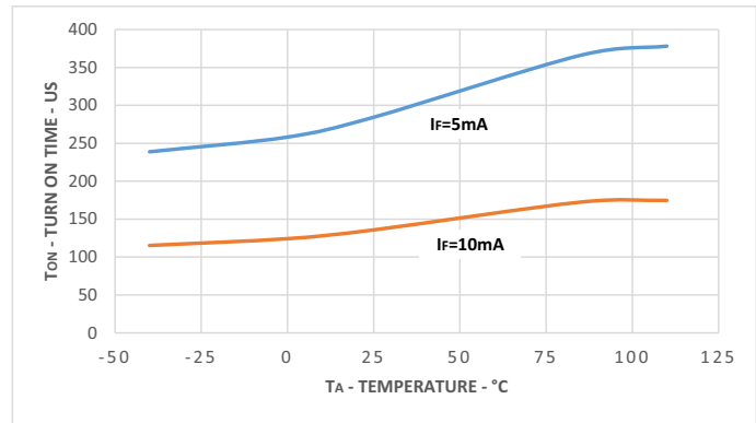
Figure 12: Typical Turn-On Time vs. Temperature
