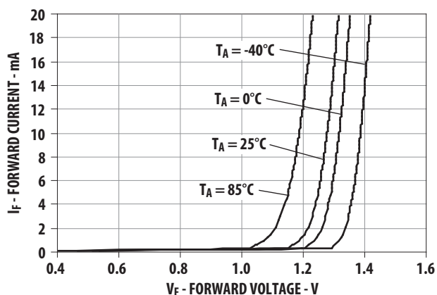
Figure 8: Typical Forward Current vs. Forward Voltage
