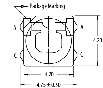
Package Drawing C
