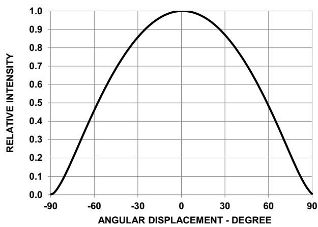
Figure 6: Radiation Pattern
