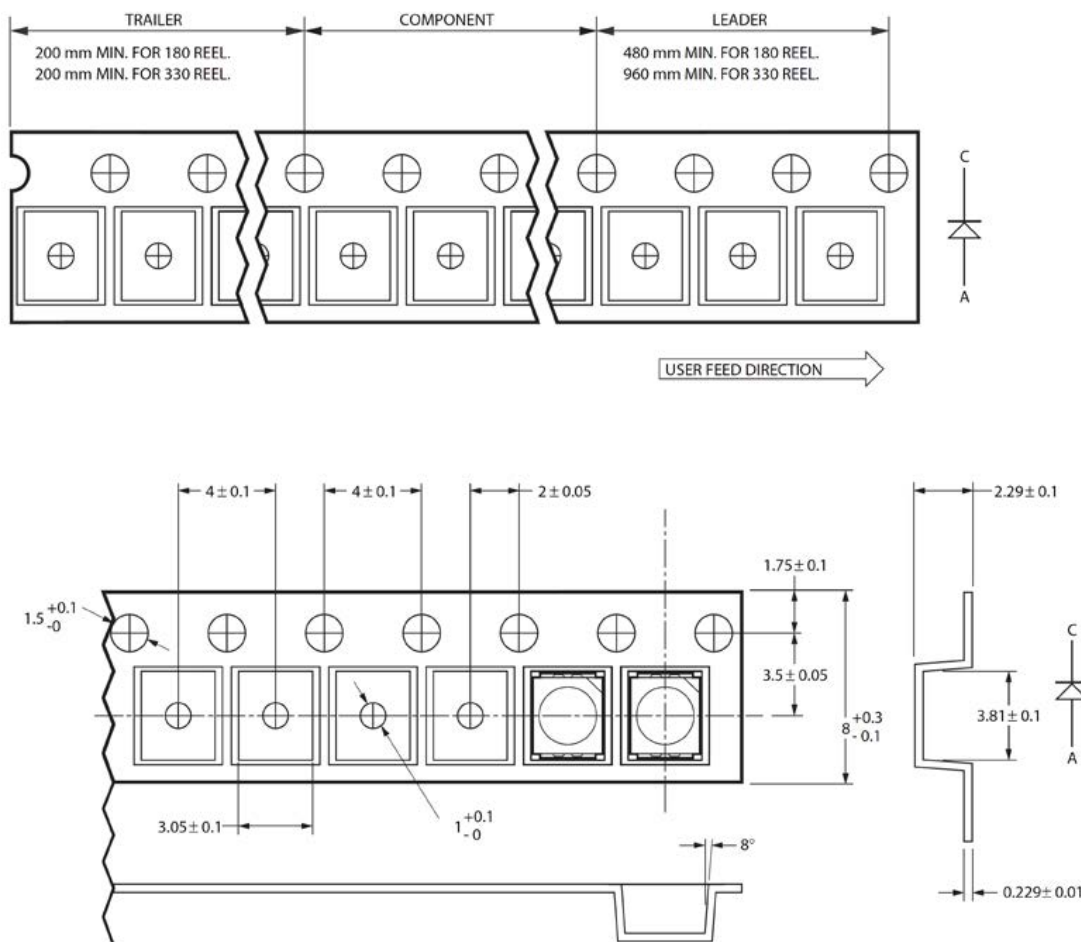
Figure 7: Carrier Tape Dimensions
