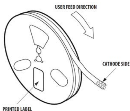
Figure 9: Reeling Orientation
