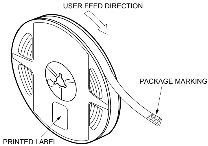
Figure 10: Reeling Orientation
