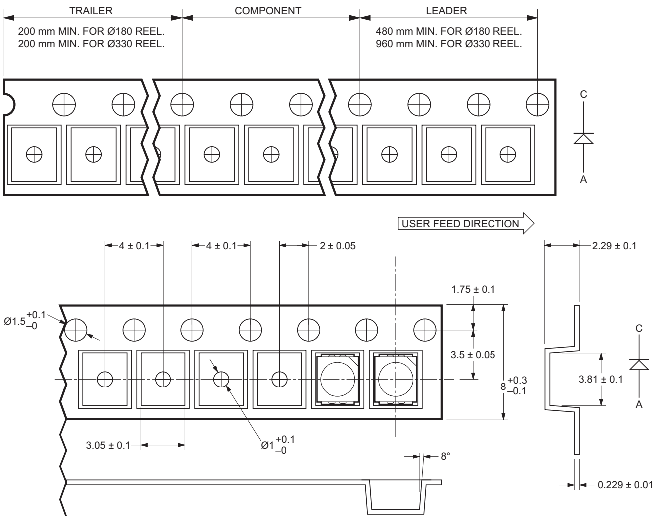
Figure 8: Carrier Tape Dimensions
