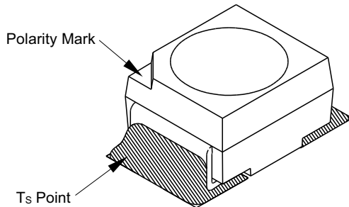
Figure 13: Solder Point Temperature on PCB
