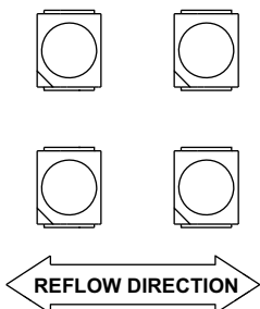
Figure 12: Recommended Board Reflow Direction
