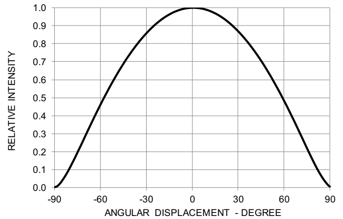
Figure 5: Radiation Pattern
