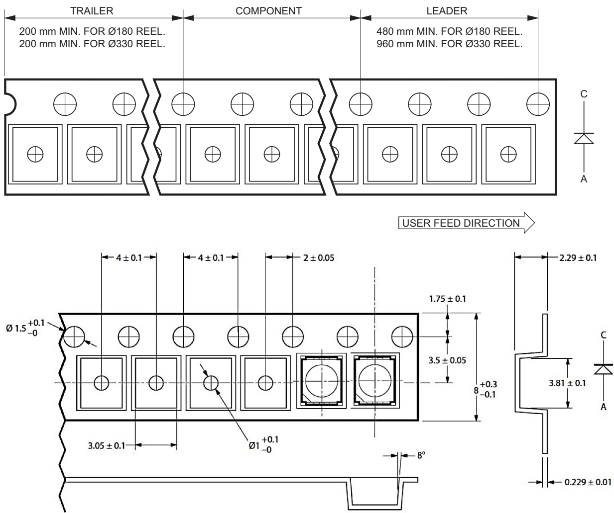
Figure 8: Carrier Tape Dimensions
