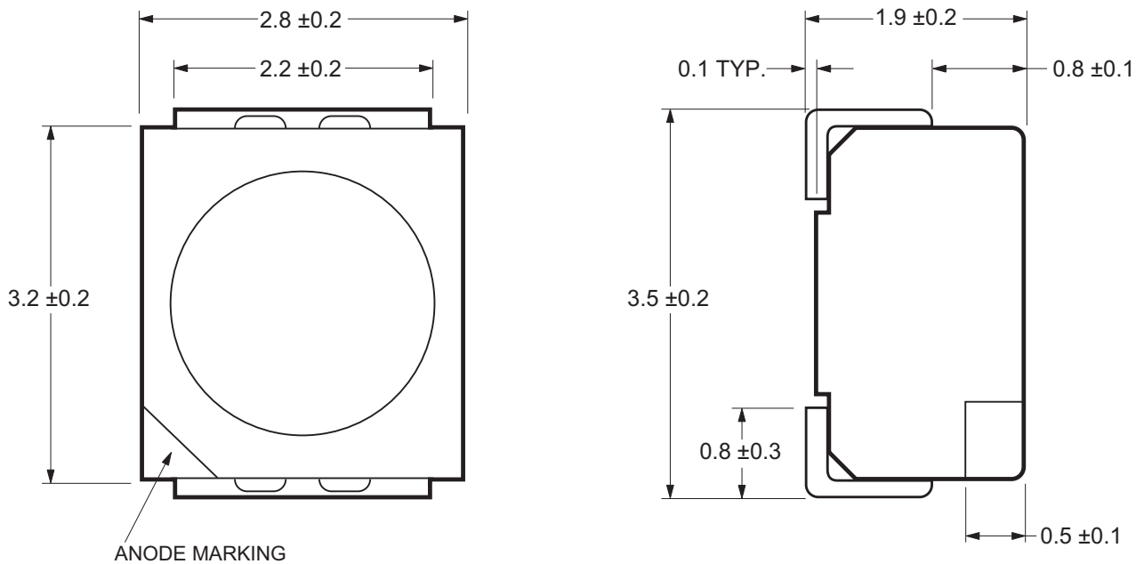
Figure 1: Package Drawing
