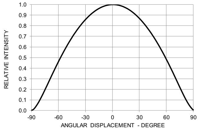
Figure 5: Radiation Pattern
