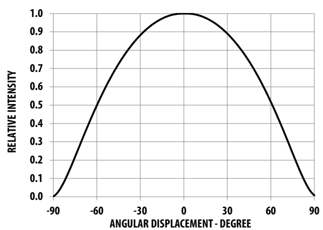
Figure 6: Radiation Pattern
