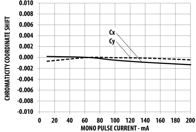
Figure 7: Chromaticity Coordinate Shift vs Forward Current for 3000K
