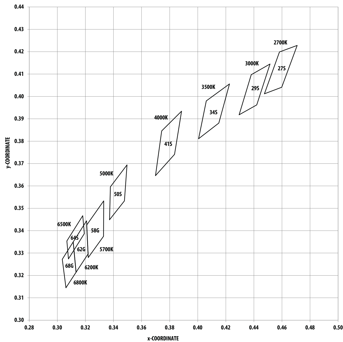
Figure 2: Chromaticity Diagram
