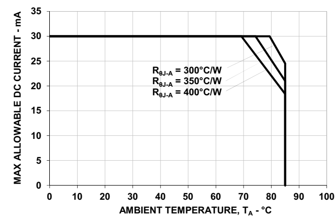
Figure 14: Maximum Forward Current vs. Ambient Temperature. Derated based on T_{JMAX} = 110^{\circ}C
