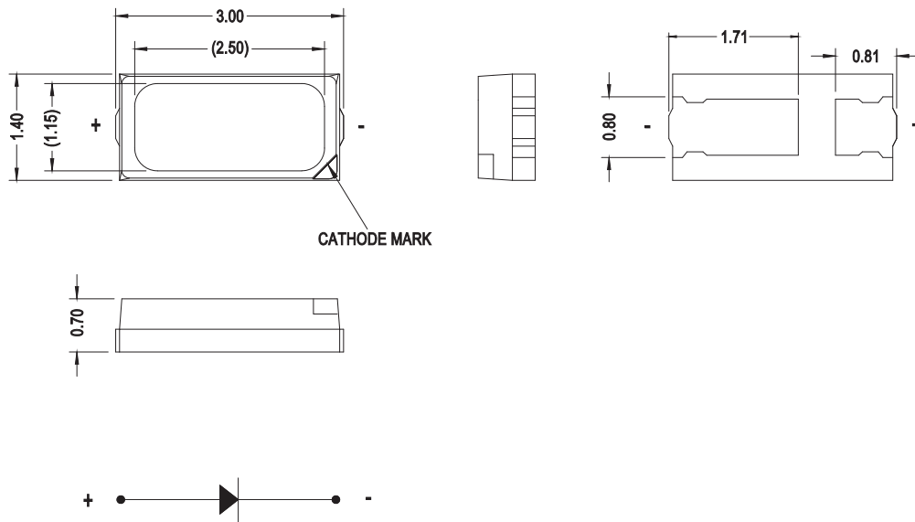
Figure 1: Package Drawing
