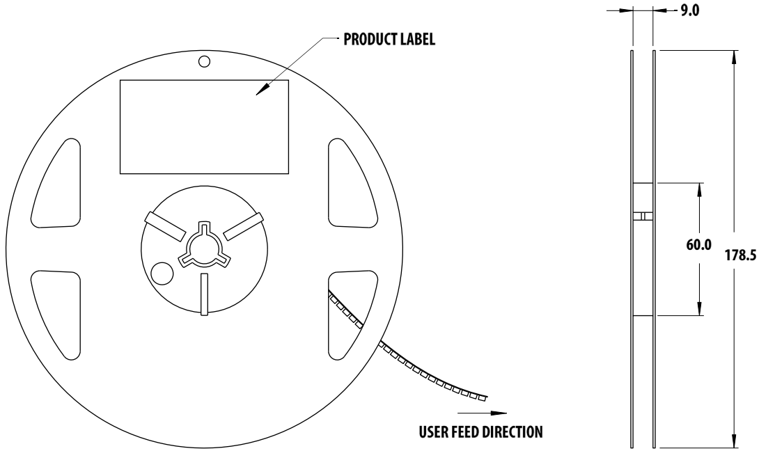
Figure 14: Reel Dimensions
