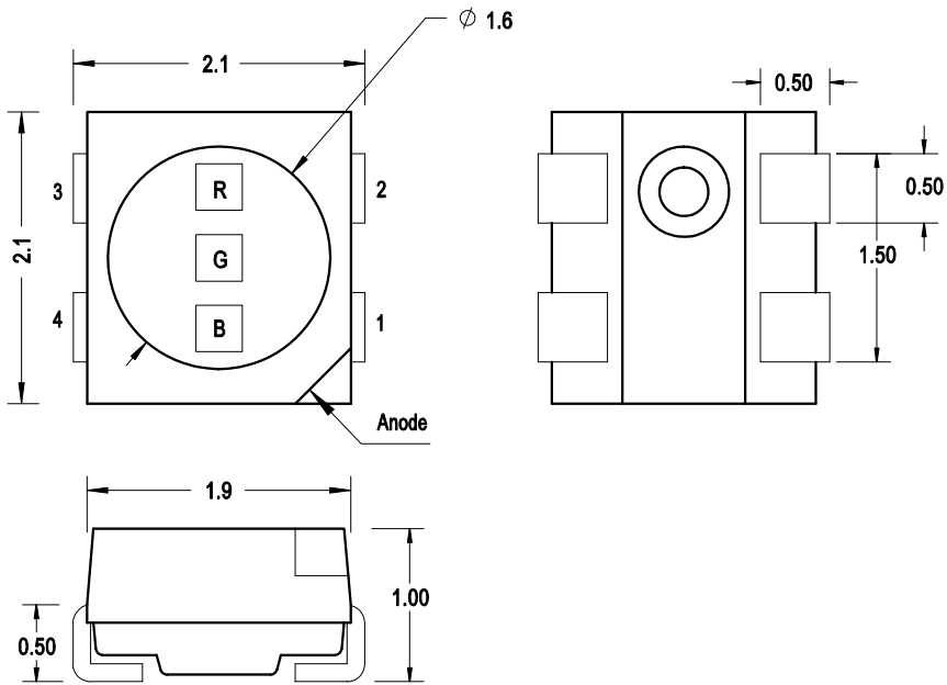
Figure 1: Package Drawing
